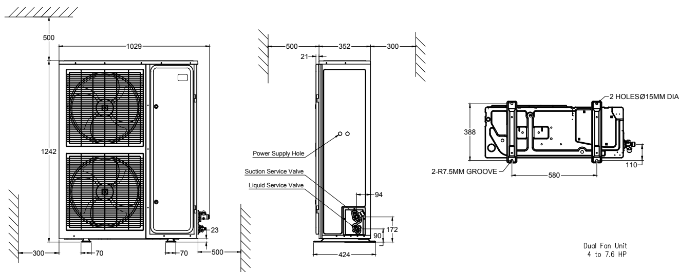
Fixing dimensions and distances - Dual fan unit
